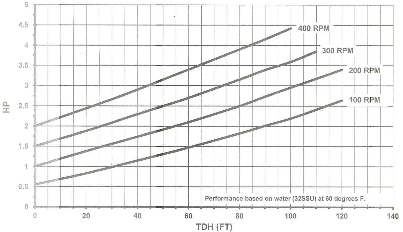
Power Consumption Curve
